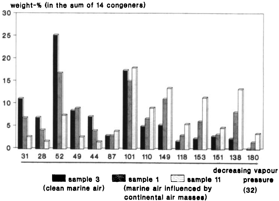
Figure 10 Comparison of the PCB patterns of a marine clean-air sample and air samples influenced by continental air masses. The PCB congeners are ordered by decreasing vapour pressures (from ref. 32).
